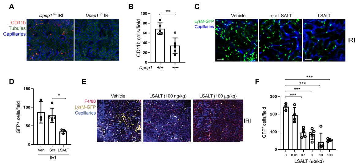
Fig. 2. DPEP1 and leukocyte recruitment during kidney IRI. (A) Kidney IVM in Dpep1 +/+ and Dpep1 -/- mice at 2 hours following renal IRI. Labels: leukocytes (CD11b, red), tubules (autofluorescence, green), and capillaries (QTracker, blue). Scale bars, 100 µm. (B) Quantification of stationary CD11b + cells/field in the kidney ( Dpep1 +/+ versus Dpep1 -/- , **P = 0.003, n = 5 to 6 per group, Student's t test). (C) Kidney IVM in LysM gfp/gfp mice 2 hours following IRI. Mice were pretreated with vehicle (phosphate-buffered saline), scrambled (Scr) LSALT peptide, or LSALT peptide. Labels: leukocytes (LysM-GFP, bright green) and capillaries (QTracker, blue). Scale bars, 50 µm. (D) Quantification of stationary GFP + leukocytes/field in the kidneys of mice 2 hours after IRI treatment with vehicle, LSALT peptide, or scrambled LSALT peptide (LSALT peptide versus scrambled peptide, *P = 0.03, n = 3 to 5). (E) Kidney IVM and (F) quantification of stationary GFP + leukocytes in LysM gfp/gfp mice 2 hours after IRI treatment with increasing doses of LSALT peptide. Labels: macrophages (F4/80, red), leukocytes (LysM-GFP, yellow), tubules (autofluorescence, dark green), and capillaries (QTracker, blue) [LSALT peptide 0 µg/kg versus 0.1 µg/kg, ***P = 0.0002; 1 µg/kg, ***P = 0.0001; 10 µg/kg, ***P = 0.0003; 100 µg/kg, ***P = 0.0001; n = 3 to 5 per group, analysis of variance (ANOVA) with Dunnett's post hoc test].
